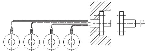
Fig. 12: SLS assembly
