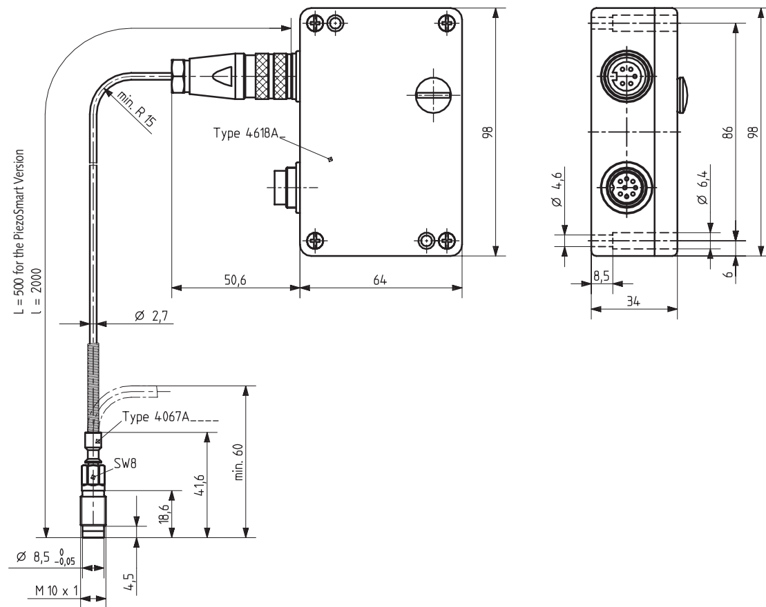
Fig. 7: Measuring chain
