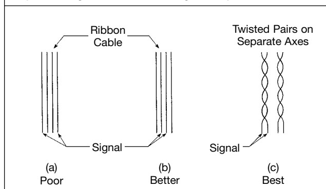
Figure 6. Cable comparison.
