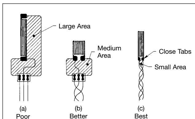
Figure 5. Gage selection and wiring technique.
